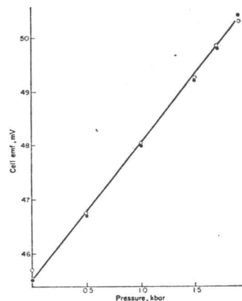
FIG. 3. Effect of temperature hysteresis on 4.5 M KCl cell at 25°C. ○, before temperature excursion to 90°C, measurements at 25°C; ●, after temperature excursion to 90°C, measurements at 25°C.
